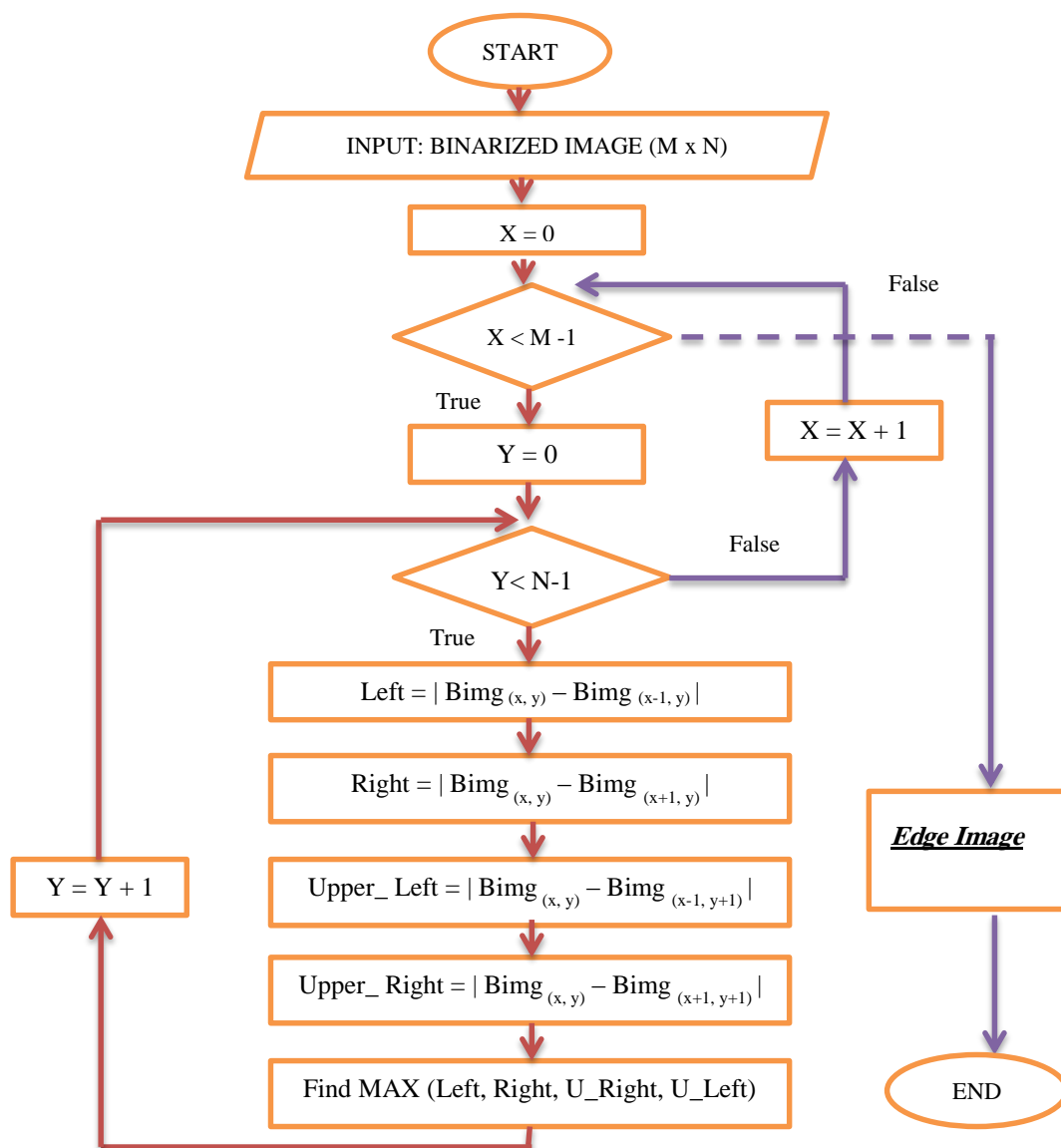
Figure 3.12 Flow Chart of Edge Detection of Character Region
